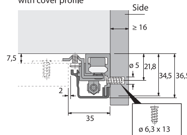
Inset with cover profile
